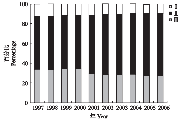
图 4 1997—2006 年城市建成区建筑物有机碳库的构成 Fig. 4 Composition of building organic carbon pools of China's urban built-up areas from 1997 to 2006.
